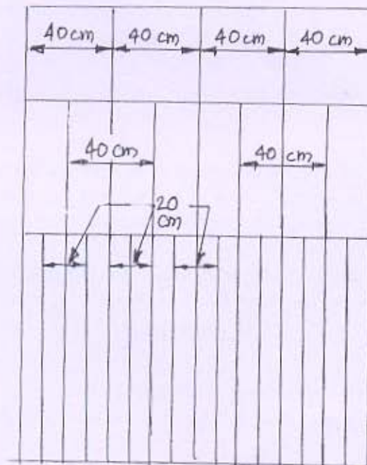
Arrangement of 20 mm \phi Main Reinforcement Bars
