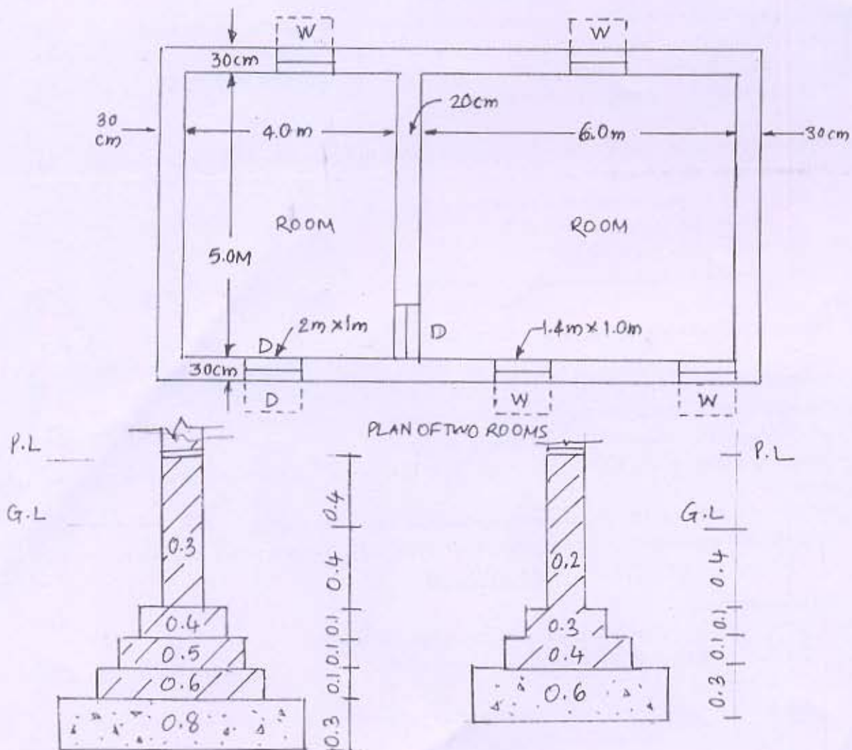
Figure 1. Two room plan with foundation detail
